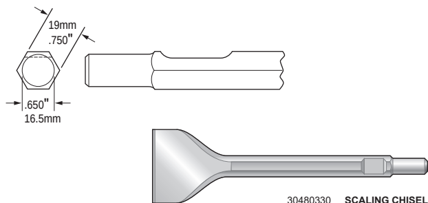
30480330 SCALING CHISEL
