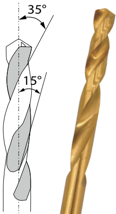
Variable helix
